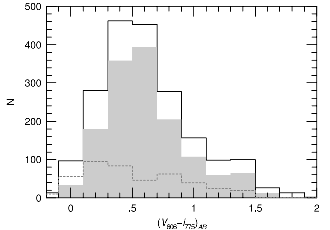
FIG. 8.— Number of galaxies placed on masks ( solid black line ), and number of redshifts measured ( grey histogram ), as a function of the V_{606} - i_{775} color. Also shown is the distribution of galaxies with redshift qualities Q = 1 and 2 ( dashed line ). For the bluest galaxies the success rate (ratio of grey histogram to solid line) is under 50%, and, as discussed in the text and Fig. 10, is likely due to unidentified high-redshift galaxies.
